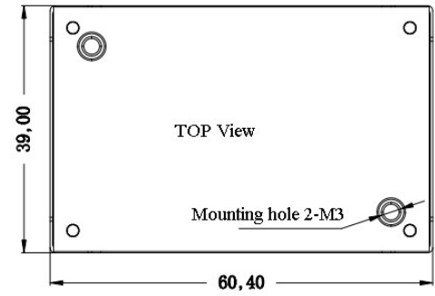
Standard 60.4*39.0*12.7mm
