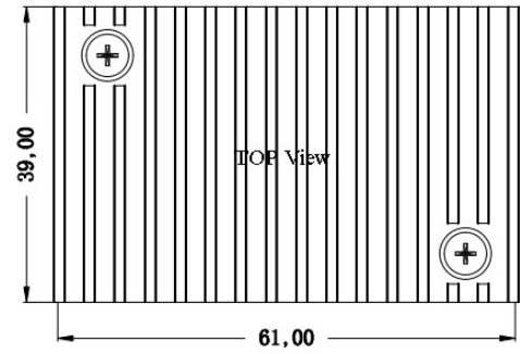
Standard+Heatsink 61.0*39.0*27.7mm
